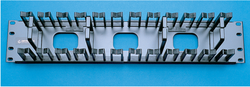
Legrand cable management panels provide organized movement of patch cables. Cable Management Panel - four horizontal - four vertical distribution rings - 2 H x 4 V cutouts - 2 rack units - 3.5 in - black
