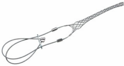
FC30LB: Bus Drop, Closed Mesh, Locking Bale, Cable Diameter 0.30 - 0.43 inches , Bale Length 12-in, Mesh Length 4.5-in, Break Strength 1100 lbs.
