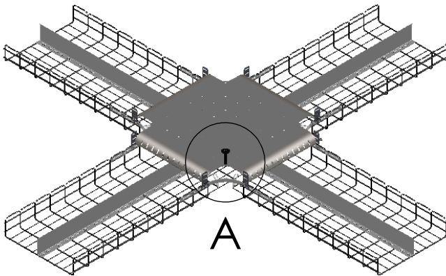
BH75 (SHOWN INSTALLED ON A HBX450 HORIZONTAL BRIDGE & CF105/450 WIRE MESH)
