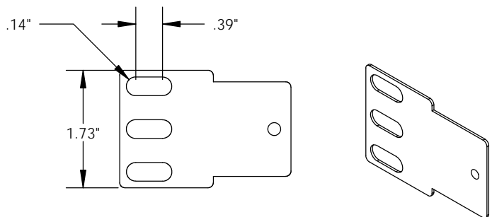
MOUNTING BRACKET (2) INCLUDED
