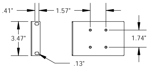
MOUNTING BRACKET (2) INCLUDED
