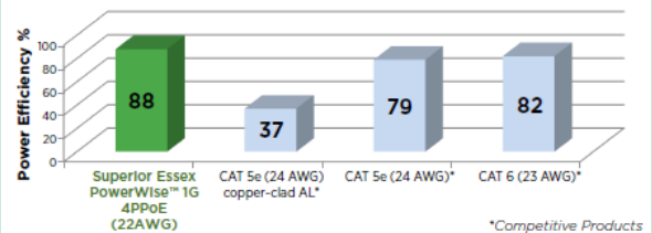
Most Energy Efficient Cable on the Market 88% Power Efficiency
