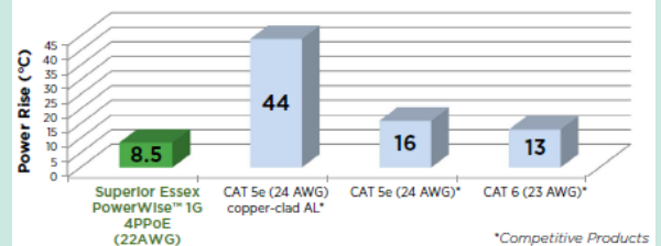
Lowest Temperature Rise via 22 AWG Conductors
