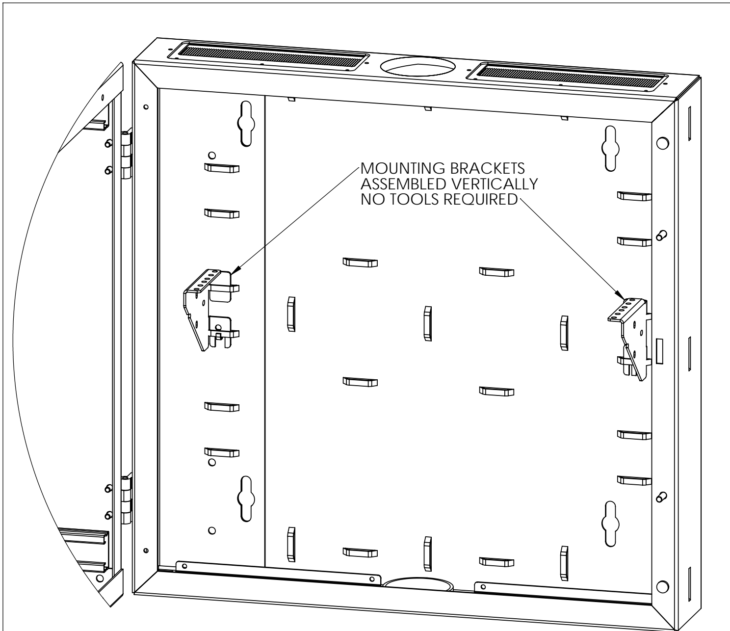
(REAR SECTION OF WALL MOUNT CABINET SHOWN, SOLD SEPERATELY)
