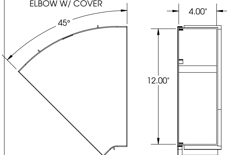
TYPICAL 45° HORIZONTAL ELBOW W/ COVER
