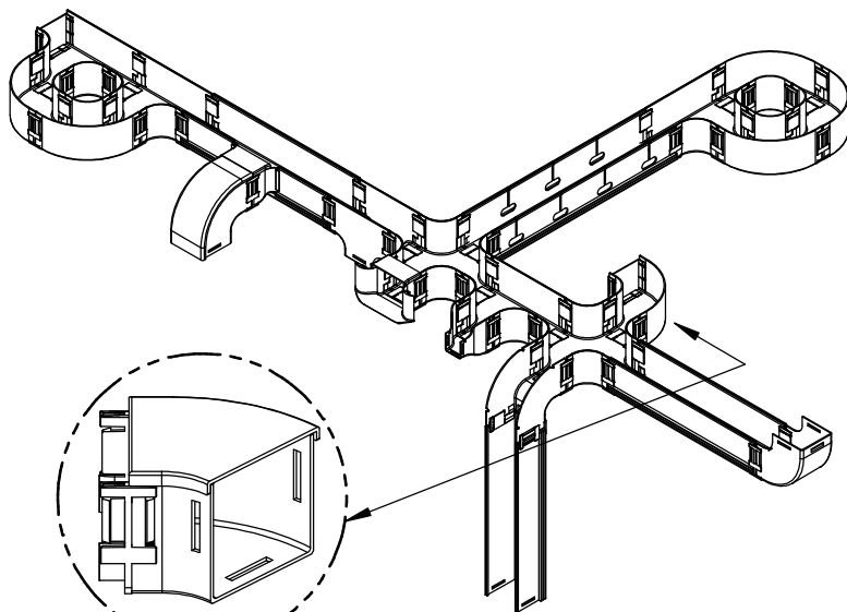
TYPICAL 45° HORIZONTAL ELBOW W/ COVER
