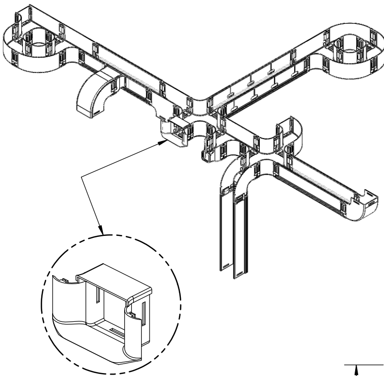
TYPICAL OUTLET TRUMPET
