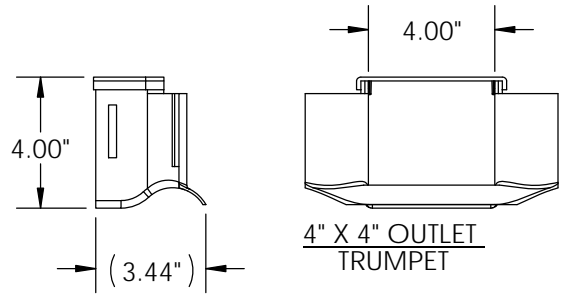
4" X 4" OUTLET TRUMPET
