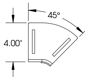
8" X 4" 45° DOWN ELBOW
