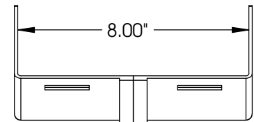
8" X 4" 45° UP ELBOW
