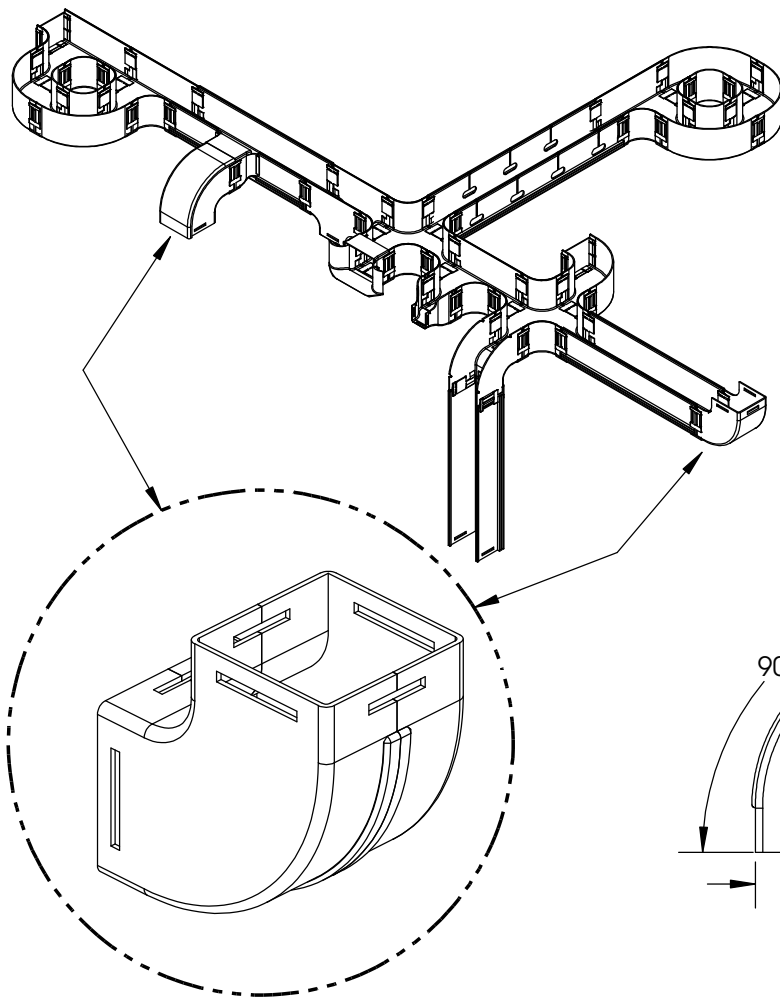
TYPICAL 90° UP/DOWN ENCLOSED ELBOW
