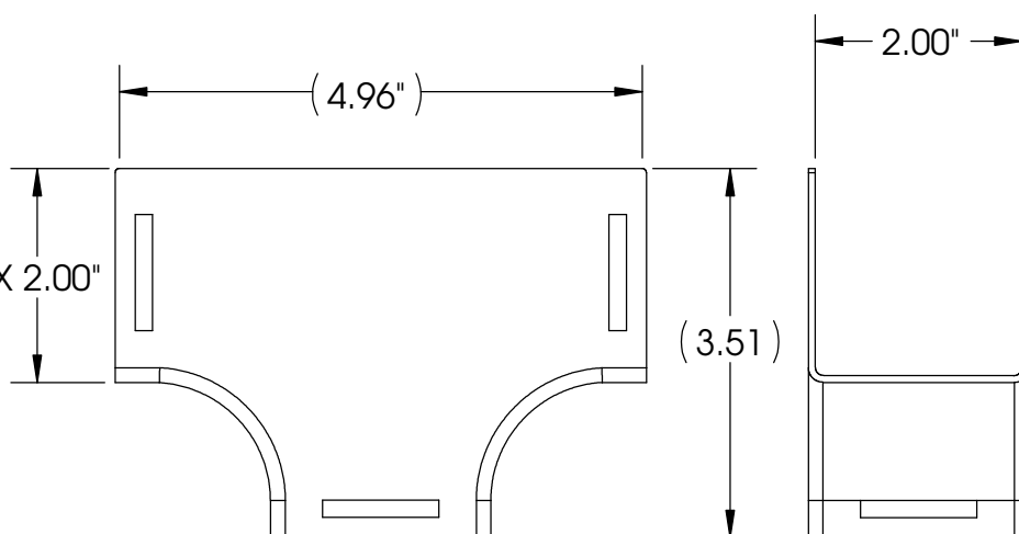
2" X 2" VERTICAL TEE TO 2" X 2" OPENING
