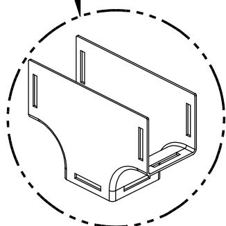
2" X 2" VERTICAL TEE
