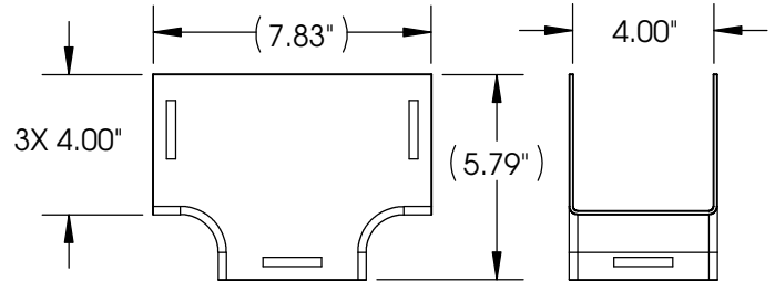
4" X 4" VERTICAL TEE TO 4" X 4" OPENING
