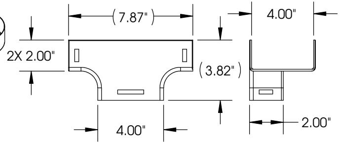
4" X 2" VERTICAL TEE TO 4" X 2" OPENING
