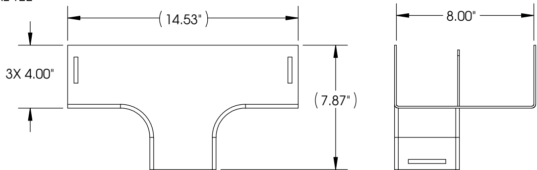
8" X 4" VERTICAL TEE TO 4" X 4" OPENING
