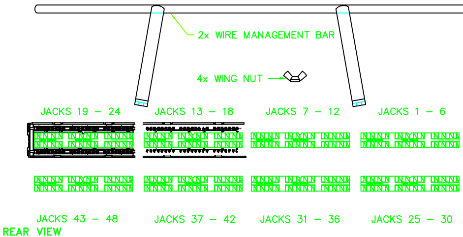
REAR VIEW
