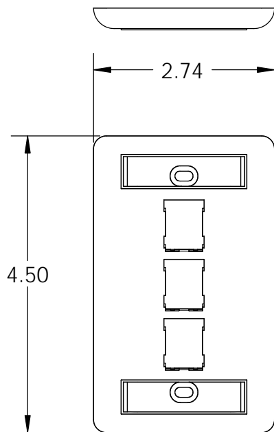
FACEPLATE (FP)
