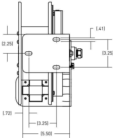
Base Mounting
