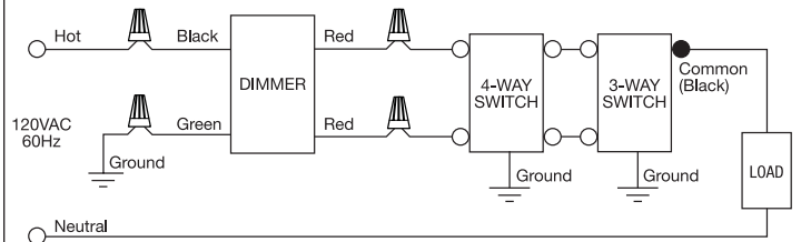
DIAGRAM 4 (4-Way Wiring)
