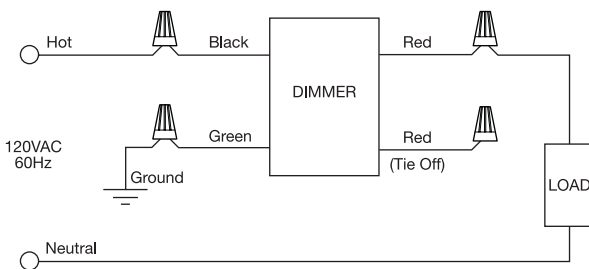
DIAGRAM 2 (Single-Pole Wiring Using 3-Way Preset Dimmer)
