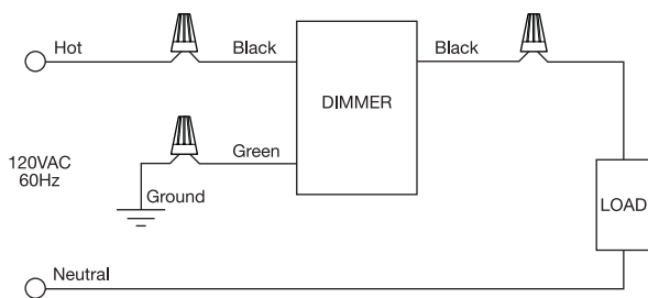
DIAGRAM 1 (Single-Pole Wiring)
