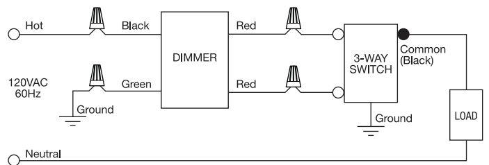
DIAGRAM 3 (3-Way Wiring)
