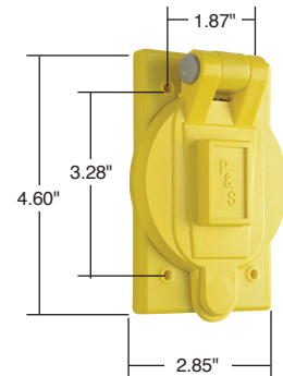
Dimensions for 7425Y
