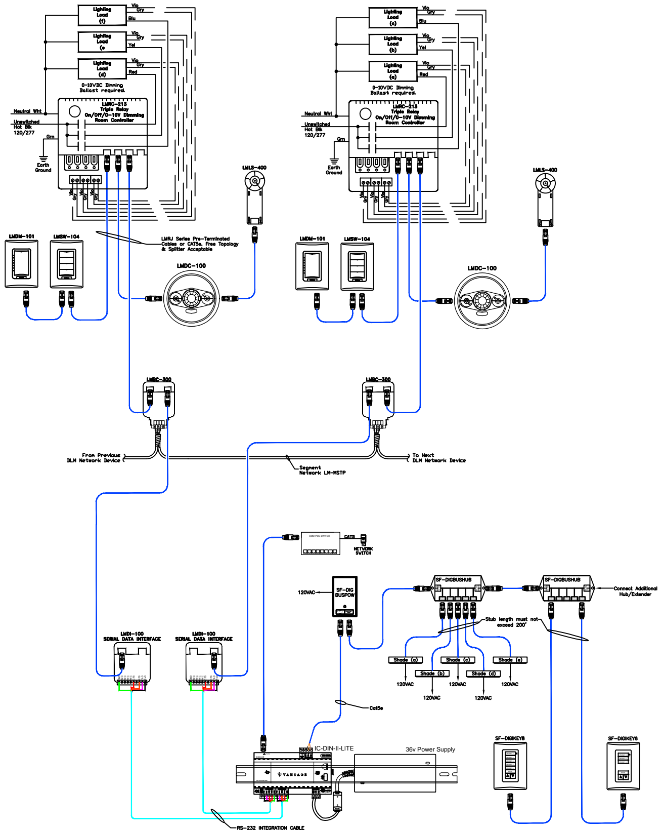
Typical DLM Digital Communication with Two Way Feedback
