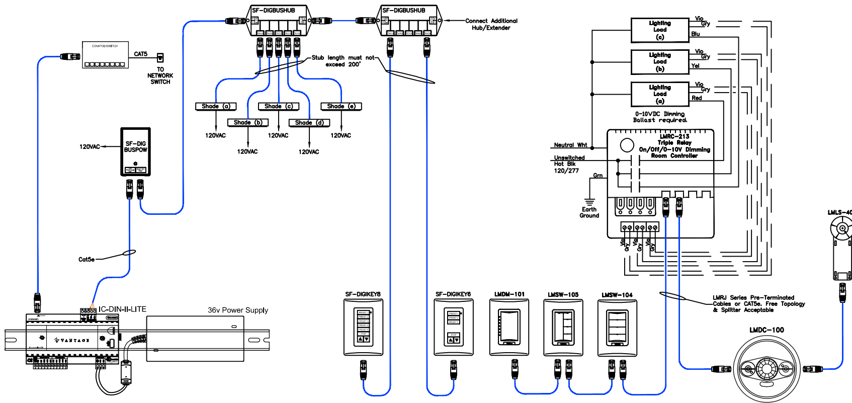
Typical Stand Alone AC Drive System with Infusion Lite Controller for Astronomical Clock Scheduling & DLM Photocell for Daylight Harvesting
