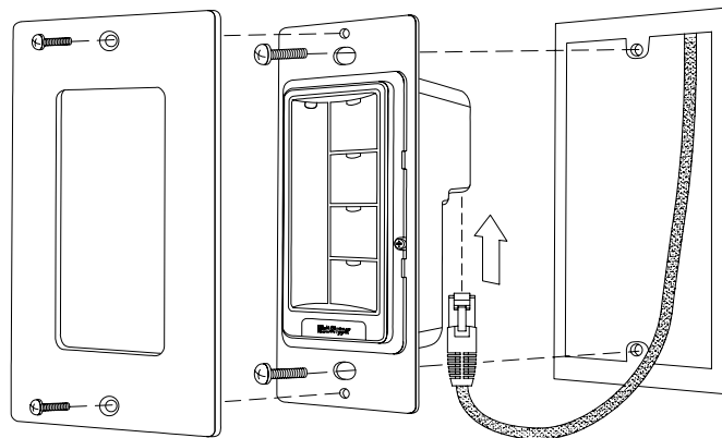
LMSW-105 Switches fit in standard single & multi gang boxes.
