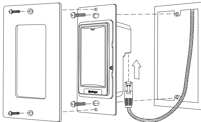
LMSW-101 Switches fit in standard single & multi gang boxes.
