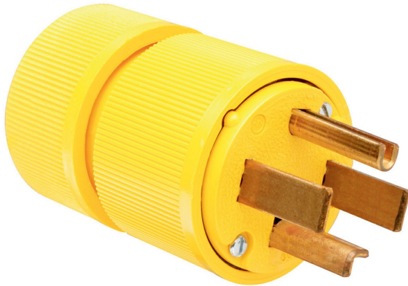
Gator Grip Plug, 3 pole 3 wire, 30A 125/250V, yellow
