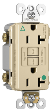
Hospital-Grade Isolated Ground Tamper-Resistant 20A Self-Test Duplex GFCI
