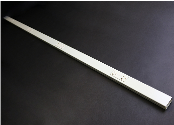
6' Steel Plugmold Multioutlet Strip with 4 duplex receptacles spaced at 18", GB
