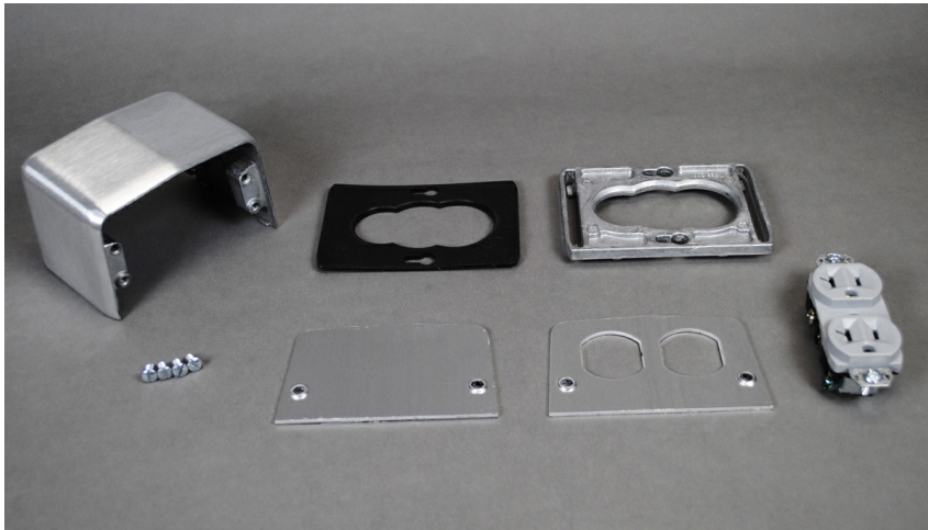
Four-piece power service fitting. 20A 125V duplex plate one side. Blank plate other side. 20A 125V receptacle included.
