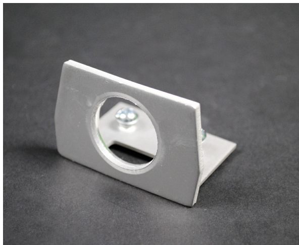
End fitting with plastic 1/2" trade size KO.
