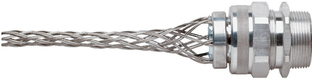
Cord Grip Male Straight, 1-1/2-inch NPT, 1.125-inch-1.250
