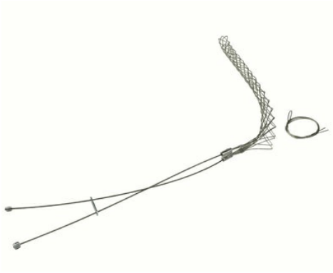
FS125LB: Standard Duty, Split Lace, Locking Bale (Universal Eye), Cable Diameter 1.25 - 1.49 inches, Bale Length 18-in, Mesh Length 16-in, Break Strength 1920 lbs.
