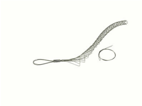
FS2000F: Standard Duty, Split Lace, Offset Eye, Cable Diameter 2.00 - 2.49 inches, Bale Length 8-in, Mesh Length 22-in
