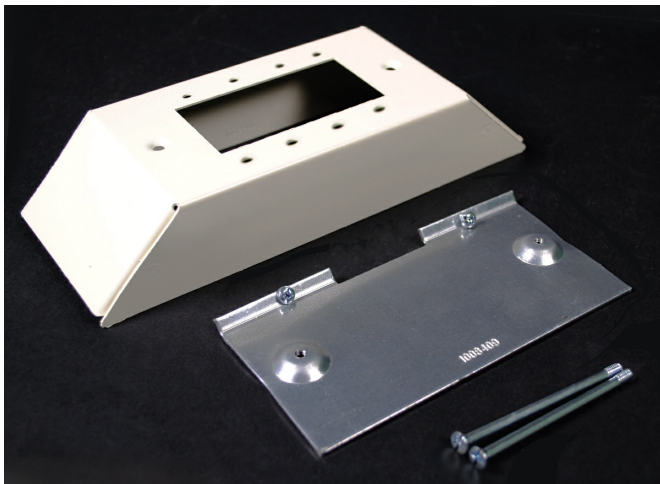
Device plate for use with four Extron Electronics MAAP single space modules.
