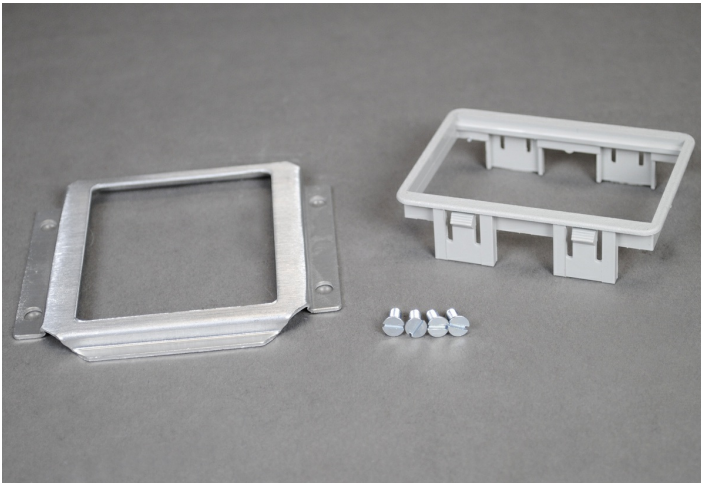
Faceplate with 6a mini adapter for Wiremold Open System CM2 communication modules.
