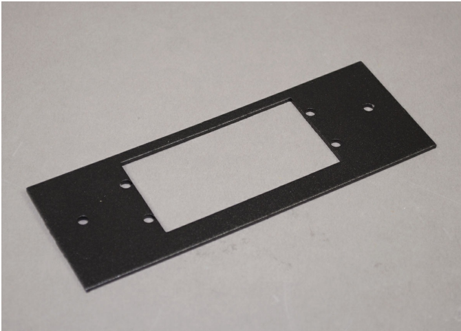
Device plate that will accept two (2) Extron Electronics AAP single space modules.
