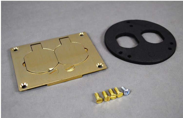
Flush brass power cover plate only (flip lid) with four mounting screws.
