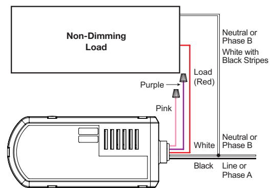
FSP-221 wiring with non-dimming load
