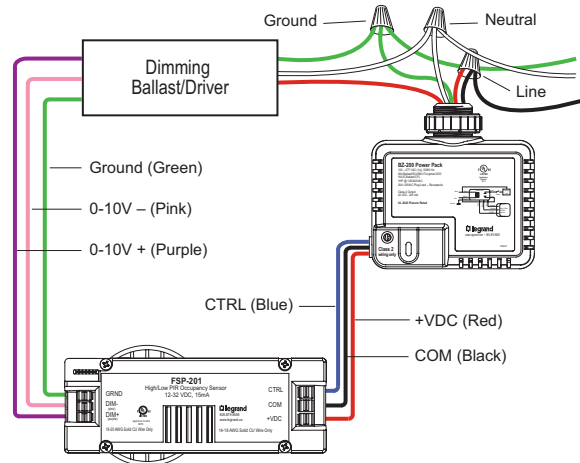
FSP-201 wiring with dimming ballast or LED driver and power pack for on/off control.
