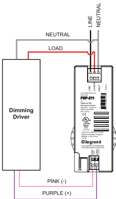
FSP-211 wiring with dimming ballast or LED driver.
