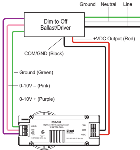
FSP-201 typical wiring with dim-to-off ballast or LED driver with auxiliary output.
