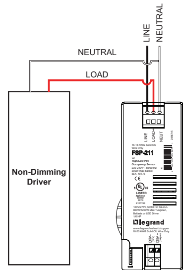
FSP-211 wiring with non-dimming ballast or LED driver.
