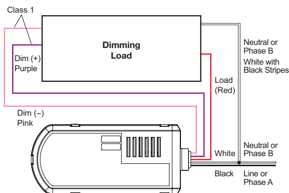
FSP-221 wiring with dimming ballast or LED driver
