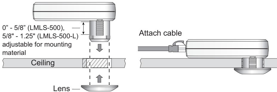
Mount Sensor to Ceiling
