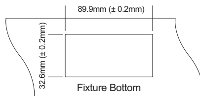
Cutout for snap-in mounting
