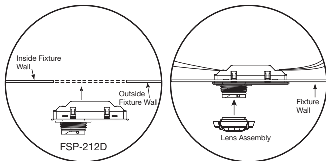
Snap-in Mounting
