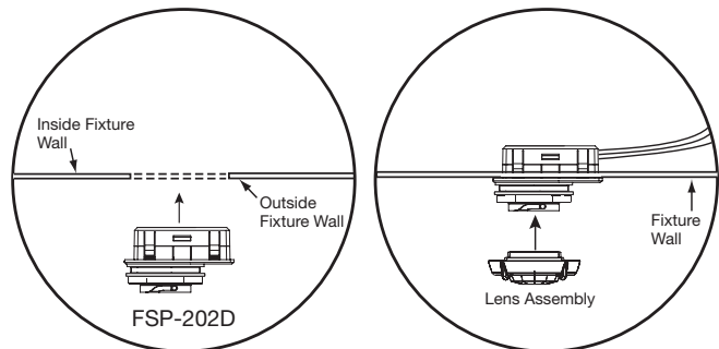
Snap-in Mounting
