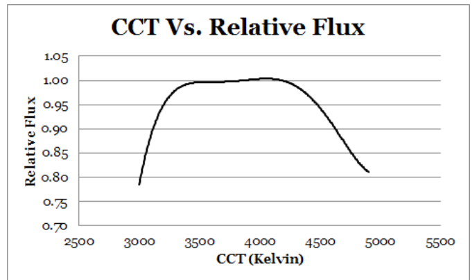
Typical relative flux at deferring correlated color temperatures
