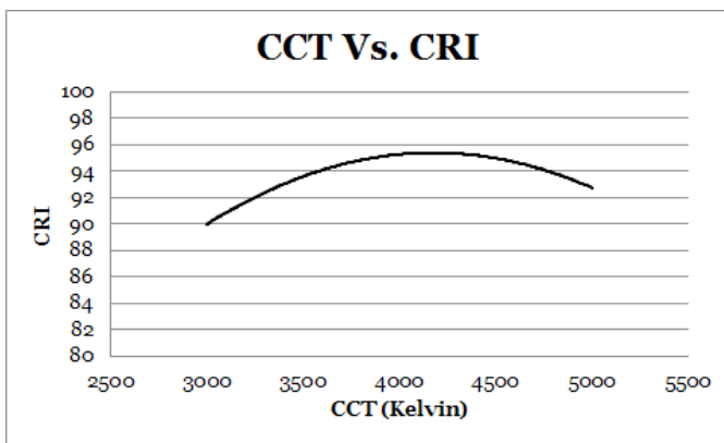
Typical CRI at deferring correlated color temperatures
