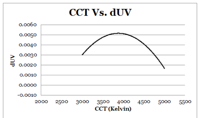
Color tolerance measured in dUV at deferring correlated color temperatures
