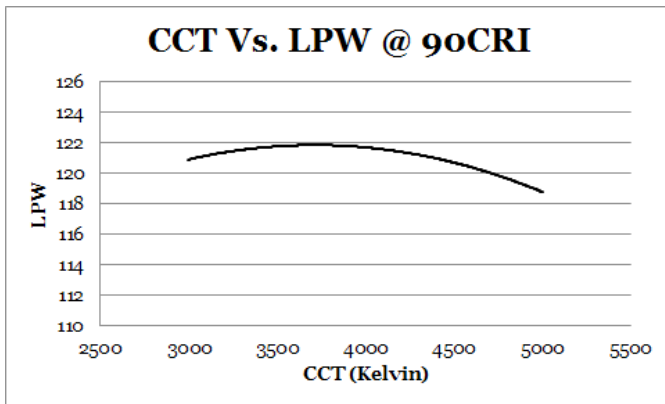
Typical lumens per watt at deferring correlated color temperatures
