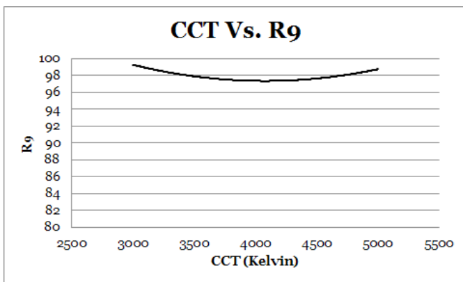
Typical R9 value at deferring correlated color temperatures
