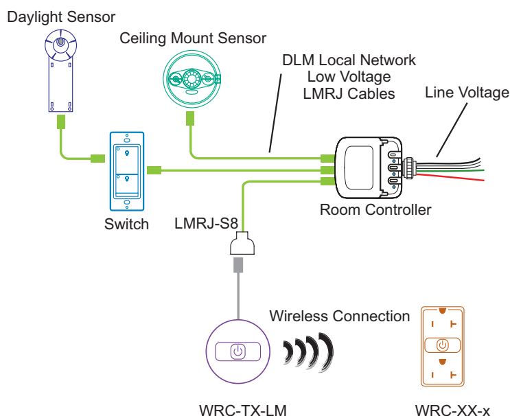
Figure 3: Connection Example
