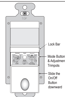
Fig. 5: Sensor Adjustment Controls
