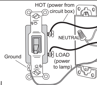
Fig. 2: Typical Single Pole Switch Wiring
