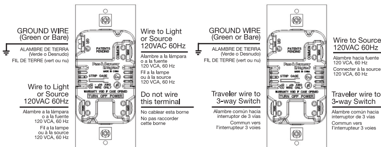
Single Pole/Unipolar/Unipolaire
