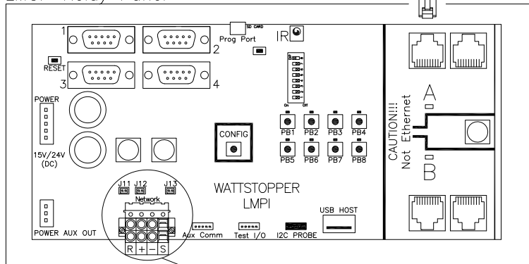
LMCP Relay Panel
