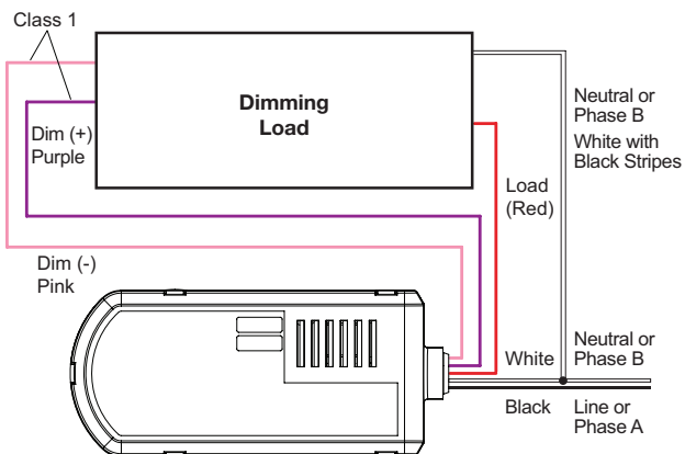
FSP-321 Dimming Wiring
