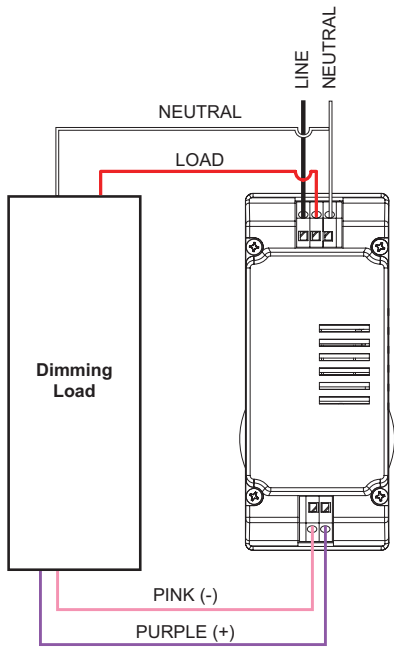
FSP-321 Dimming Wiring
