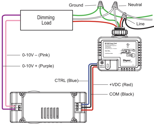
FSP-301 Wiring with Power Pack
