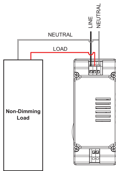
FSP-311 Non-Dimming Wiring
