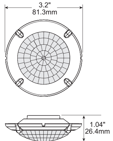
FSP-L7 dimensions
