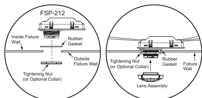
Figure 2. Installing the FSP-212D in the light fixture
