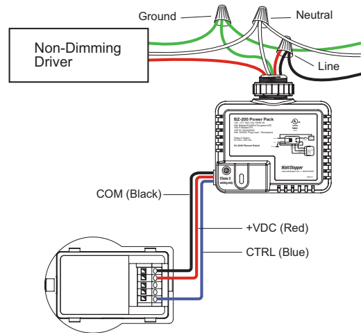
Figure 4. FSP-202D wiring with non-dimming ballast or LED driver and power pack for on/off control
