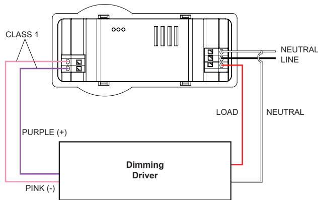
Figure 7. FSP-212D wiring with dimming ballast or LED driver
