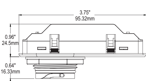
FSP-212D dimensions
