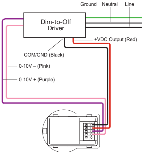
Figure 3. FSP-202D wiring with dim-to-off ballast or LED driver
