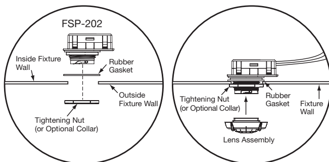
Figure 1. Installing the FSP-202D in the light fixture
