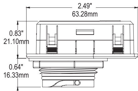
FSP-202D dimensions
