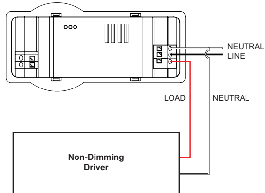
Figure 8. FSP-212D wiring with non-dimming load
