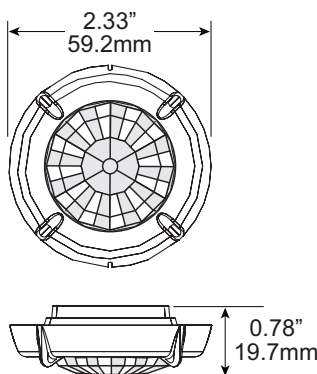
FSP-L3 dimensions
